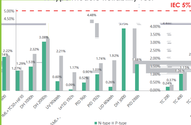
N-type Module Reliability Test
